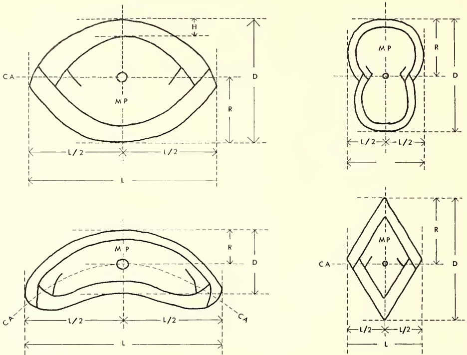
TEXT-FIG. 2. Operational definitions of morphological terms for various shapes of test: diameter (D), radius (R), chamber-height (H), length (L), half-length (L/2), median plane (MP), coiling axis (CA).
